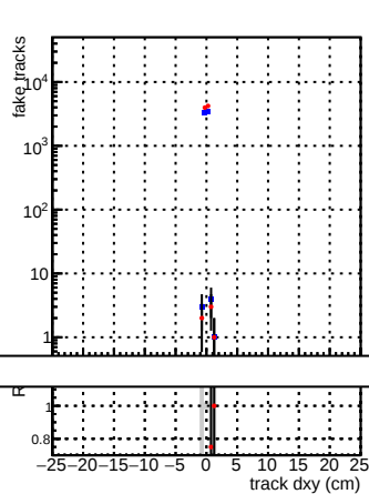
N of associated (recoToSim) loopier tracks vs dxy
