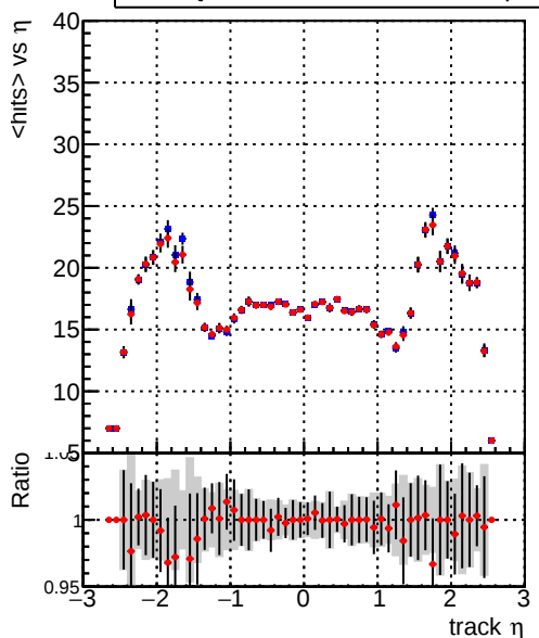
mean hits vs \eta Legend: DQM_mkFit_TTbase (blue line), DQM_mkFit_TT_retrainOldFiles125_v2_prelimWP_5iter (red line)
