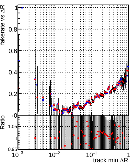
Legend: DQM_mkFit_TTbase (blue squares), DQM_mkFit_TT_retrainOldFiles125_v2_prelimWP_5iter (red circles)
