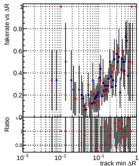
Fake rate vs \Delta R(\text{track, jet}) —•— DQM_mkFit_TTbase —•— DQM_mkFit_TT_retrainOldFiles125_v2_prelimWP_5iter
