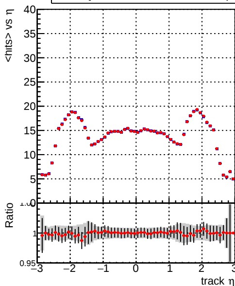
mean hit Legend: DQM_mkFit_TTbase (blue line with dots), DQM_mkFit_TT_retrainOldFiles125_v2_prelimWP_5iter (red line with dots)
