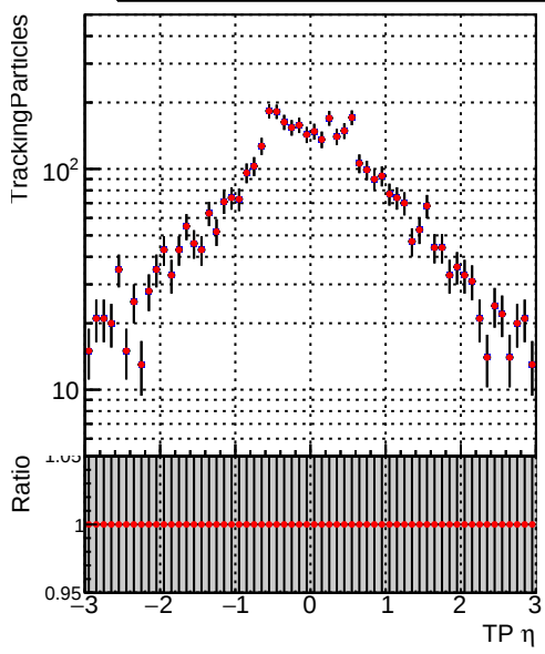
N of simulated tracks vs TP \eta Legend: DQM_mkFit_TTbase (blue dots), DQM_mkFit_TT_retrainOldFiles125_v2_prelimWP_5iter (red dots)
