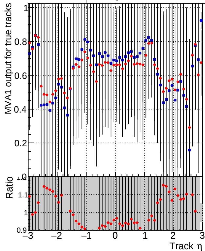
MVA1 of associated tracks (recoToSim) vs. track \eta Legend: DQM_mkFit_TTbase (blue squares) DQM_mkFit_TT_retrainOldFiles125_v2_prelimWP_5iter (red diamonds)
