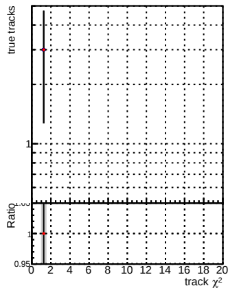
N of reco track vs. \chi^2 —•— DQM_mkFit_TTbase —•— DQM_mkFit_TT_retrainOldFiles125_v2_prelimWP_5iter
