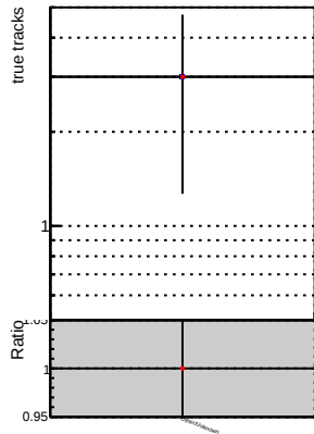
N of reco track vs. \chi^2 —•— DQM_mkFit_TTbase —•— DQM_mkFit_TT_retrainOldFiles125_v2_prelimWP_5iter
