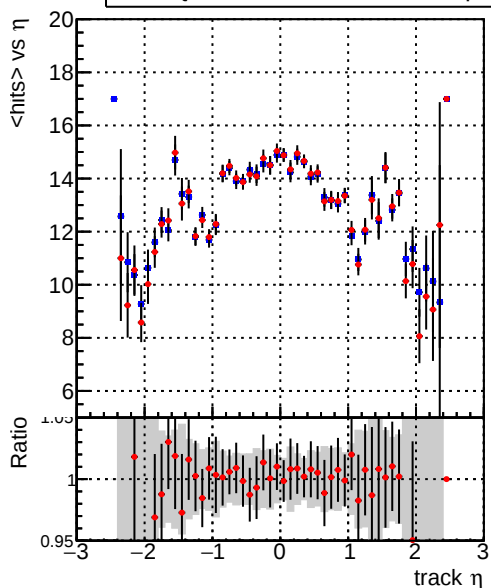
mean hits vs \eta Legend: DQM_mkFit_TTbase (blue line), DQM_mkFit_TT_retrainOldFiles125_v2_prelimWP_5iter (red line)
