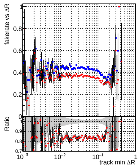
Fake rate vs \Delta R (track, jet) Legend: —•— DQM_mkFit_TTbase —•— DQM_mkFit_TT_retrainOldFiles125_v2_prelimWP_5iter
