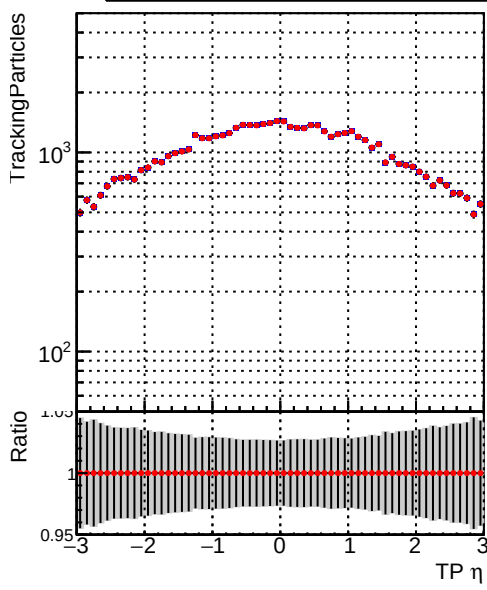
N of simulated tracks vs \eta Legend: \blacksquare DQM_mkFit_TTbase \star DQM_mkFit_TT_retrainOldFiles125_v2_prelimWP_5iter
