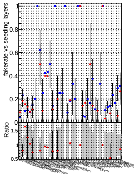
Fake rate vs. —♦— DQM_mkFit_TTbase —•— DQM_mkFit_TT_retrainOldFiles125_v2_prelimWP_5iter
