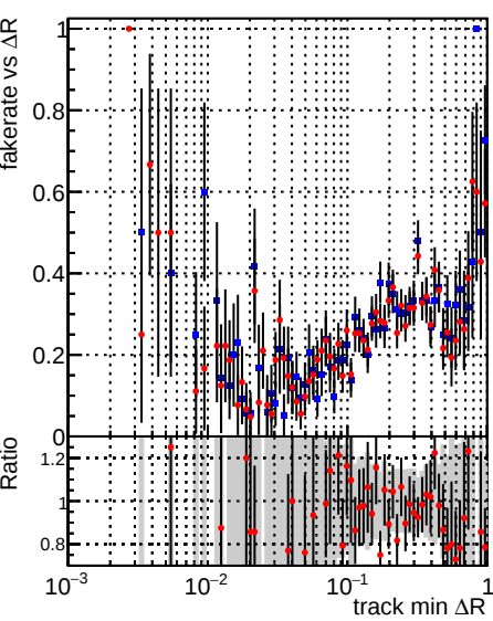
Legend: DQM_mkFit_TTbase (blue line with dots), DQM_mkFit_TT_retrainOldFiles125_v2_prelimWP_5iter (red line with dots)
