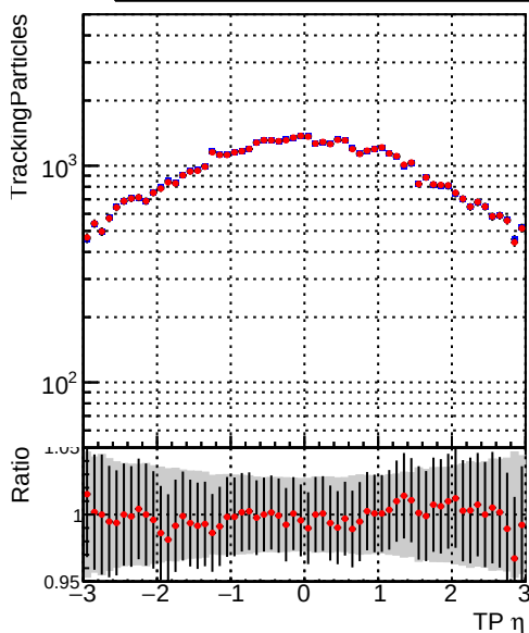
Legend: DQM_mkFit_TTbase (blue squares), DQM_mkFit_TT_retrainOldFiles125_v2_prelimWP_5iter (red circles)
