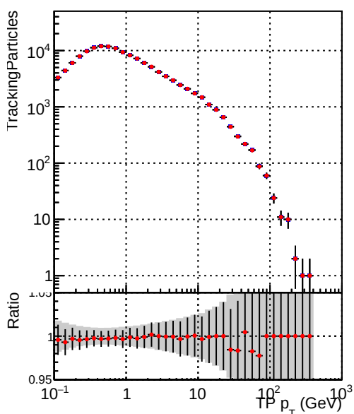
Legend: DQM_mkFit_TTbase (blue squares), DQM_mkFit_TT_retrainOldFiles125_v2_prelimWP_5iter (red circles)
