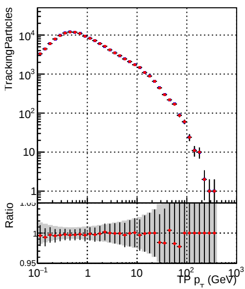
Legend: DQM_mkFit_TTbase (blue squares), DQM_mkFit_TT_retrainOldFiles125_v2_prelimWP_5iter (red crosses)
