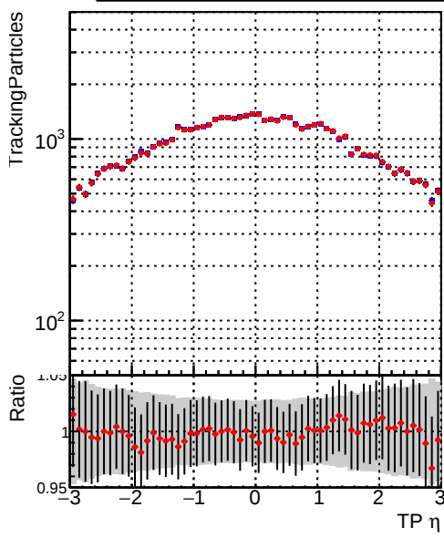
Legend: DQM_mkFit_TTbase (blue squares), DQM_mkFit_TT_retrainOldFiles125_v2_prelimWP_5iter (red crosses)
