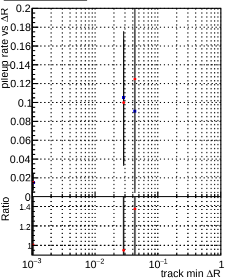
Legend: DQM_mkFit_TTbase (blue), DQM_mkFit_TT_retrainOldFiles125_v2_prelimWP_5iter (red)
