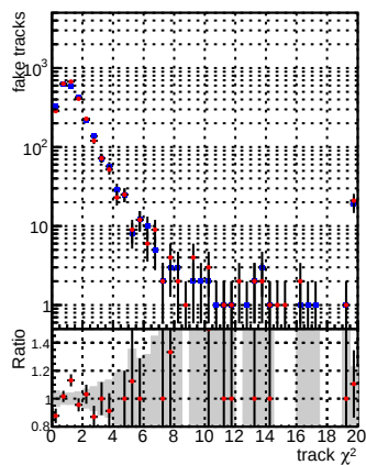
fake tracks vs. \chi^2
