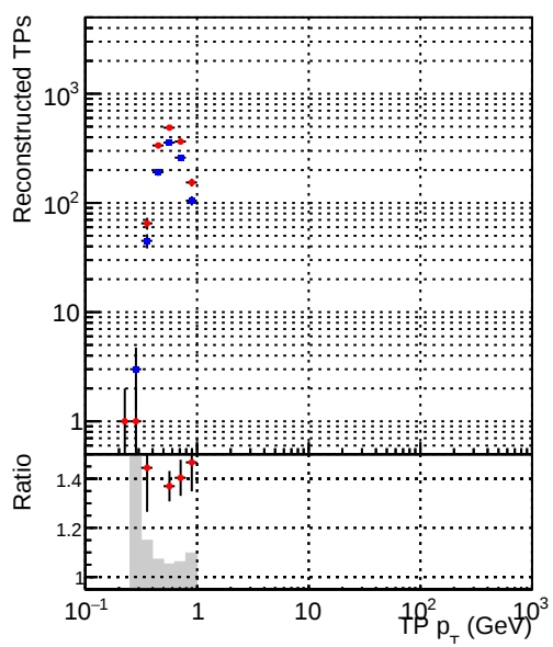
Legend: DQM_mkFit_TTbase (blue dots), DQM_mkFit_TT_retrainOldFiles125_v2_prelimWP (red dots)
