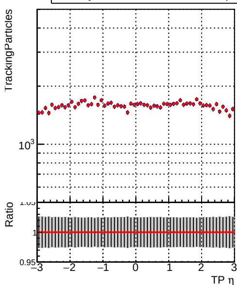
N of simulated tracks vs \eta Legend: - \blacksquare DQM_mkFit_TTbase - \bullet DQM_mkFit_TT_retrainOldFiles125_v2_prelimWP
