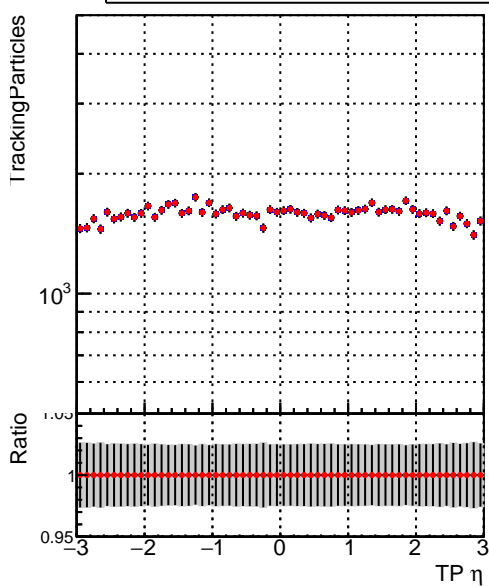
N of simulated tracks vs \eta Legend: DQM_mkFit_TTbase (blue circles), DQM_mkFit_TT_retrainOldFiles125_v2_prelimWP (red circles)
