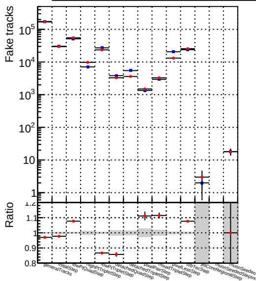
Number —●— DQM_mkFit_TT_retrainOldFiles125_v2_prelimWP
