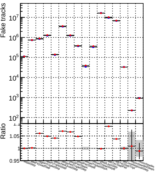
Number —●— DQM_mkFit_TT_retrainOldFiles125_v2_prelimWP
