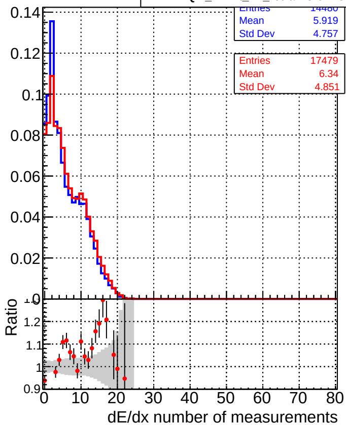
—■— DQM_mkFit_TTbase —●— DQM_mkFit_TT_retrainOldFiles125_v2_prelimWP
