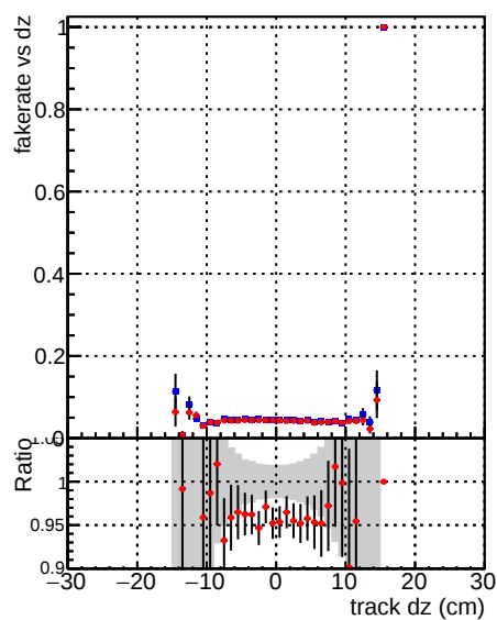
Fake rate vs dz —●— DQM_mkFit_TTbase —●— DQM_mkFit_TT_retrainOldFiles125_v2_prelimWP
