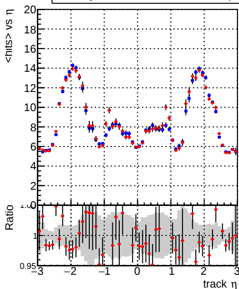
Legend: — DQM_mkFit_TTbase — DQM_mkFit_TT_retrainOldFiles125_v2_prelimWP mean hits
