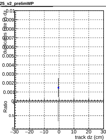
—•— DQM_mkFit_TTbase —•— DQM_mkFit_TT_retrainOldFiles125_v2_prelimWP
