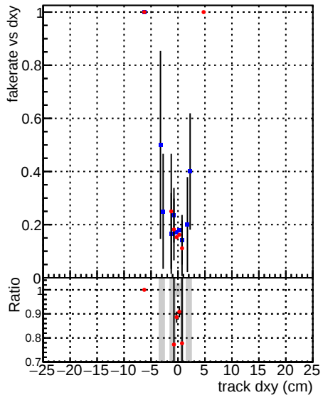
—•— DQM_mkFit_TTbase —•— DQM_mkFit_TT_retrainOldFiles125_v2_prelimWP
