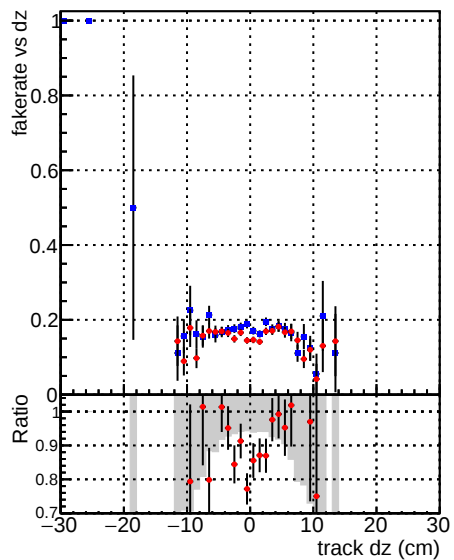
—•— DQM_mkFit_TTbase —•— DQM_mkFit_TT_retrainOldFiles125_v2_prelimWP
