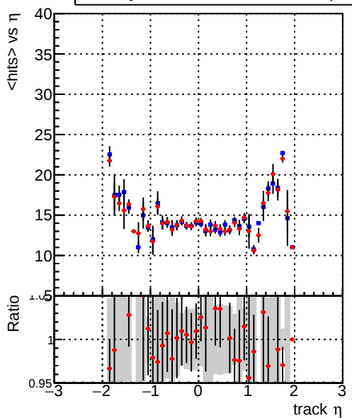
mean hits vs \eta Legend: DQM_mkFit_TTbase (blue line), DQM_mkFit_TT_retrainOldFiles125_v2_prelimWP (red line)
