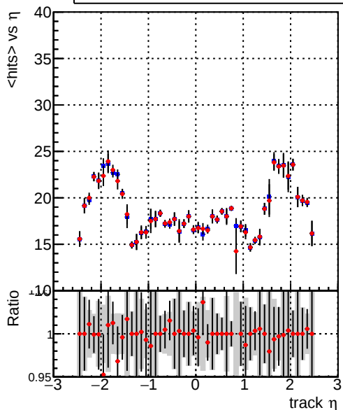
mean hits — DQM_mkFit_TTbase — DQM_mkFit_TT_retrainOldFiles125_v2_prelimWP
