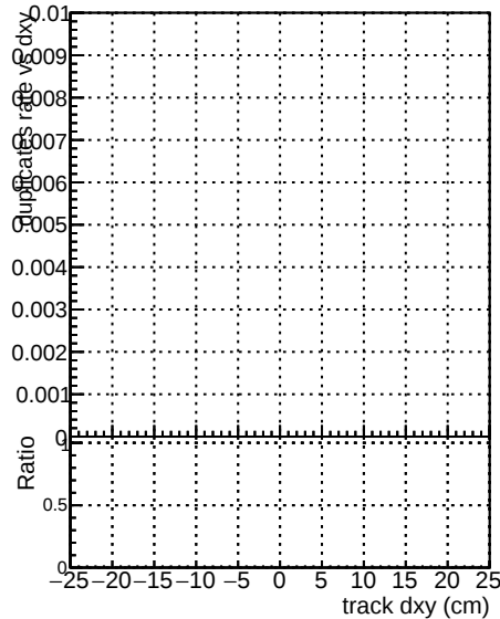
—•— DQM_mkFit_TTbase —•— DQM_mkFit_TT_retrainOldFiles125_v2_prelimWP
