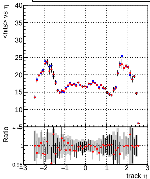
mean hits Legend: DQM_mkFit_TTbase (blue line), DQM_mkFit_TT_retrainOldFiles125_v2_prelimWP (red line)
