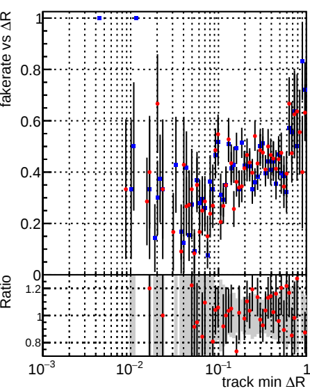
Legend: DQM_mkFit_TTbase (blue stars), DQM_mkFit_TT_retrainOldFiles125_v2_prelimWP (red stars)
