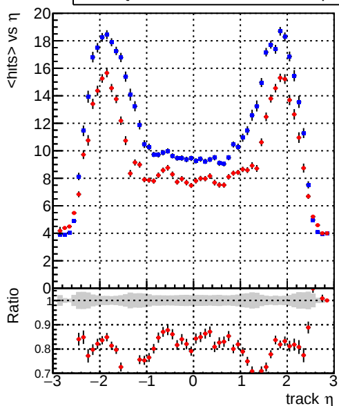
mean hit — DQM_mkFit_TTbase — DQM_mkFit_TT_retrainOldFiles125_v2_prelimWP
