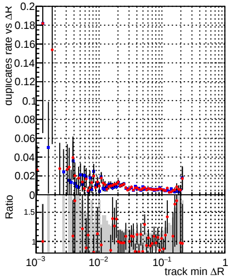
—•— DQM_mkFit_TTbase —•— DQM_mkFit_TT_retrainOldFiles125_v2_prelimWP
