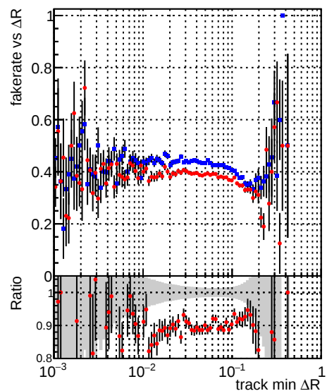
—•— DQM_mkFit_TTbase —•— DQM_mkFit_TT_retrainOldFiles125_v2_prelimWP
