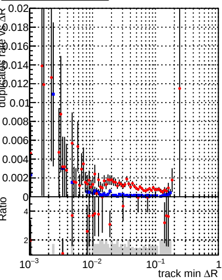
—•— DQM_mkFit_TTbase —•— DQM_mkFit_TT_retrainOldFiles125_v2_prelimWP
