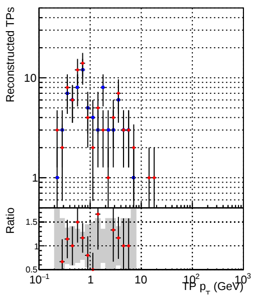
—•— DQM_mkFit_TTbase —•— DQM_mkFit_TT_retrainOldFiles125_v2_prelimWP
