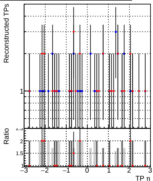
—•— DQM_mkFit_TTbase —•— DQM_mkFit_TT_retrainOldFiles125_v2_prelimWP
