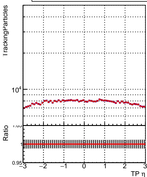
N of simulated tracks vs \eta Legend: DQM_mkFit_TTbase (blue line), DQM_mkFit_TT_retrainOldFiles125_v2_prelimWP (red line)
