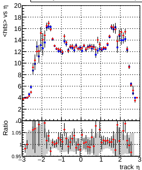
— DQM_mkFit_TTbase — DQM_mkFit_TT_retrainOldFiles125_v2_prelimWP mean hits
