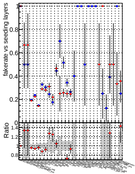
Fake rate vs. —•— DQM_mkFit_TTbase —•— DQM_mkFit_TT_retrainOldFiles125_v2_prelimWP
