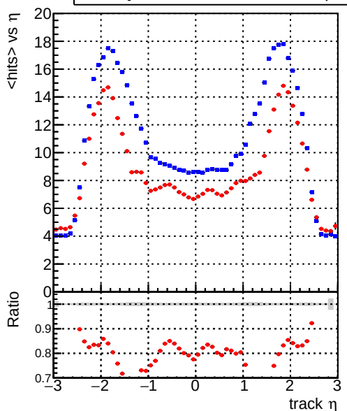
mean hit — DQM_mkFit_TTbase — DQM_mkFit_TT_retrainOldFiles125_v2_prelimWP
