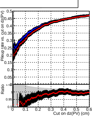
Fake rate
