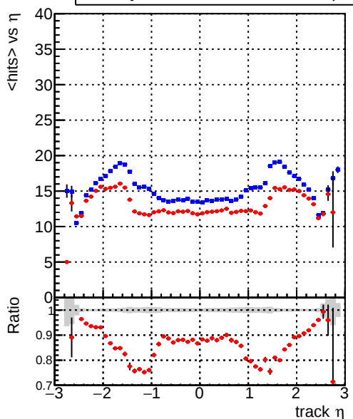
— DQM_mkFit_TTbase — DQM_mkFit_TT_retrainOldFiles125_v2_prelimWP mean hits > \eta
