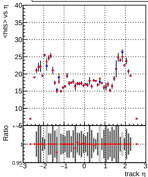
mean hits vs \eta — DQM_mkFit_TTbase — DQM_mkFit_TT_retrainOldFiles125_v2_prelimWP
