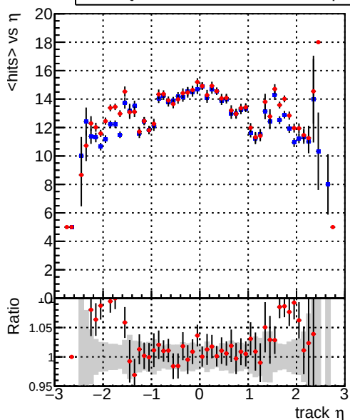
mean hits vs \eta — DQM_mkFit_TTbase — DQM_mkFit_TT_retrainOldFiles125_v2_prelimWP
