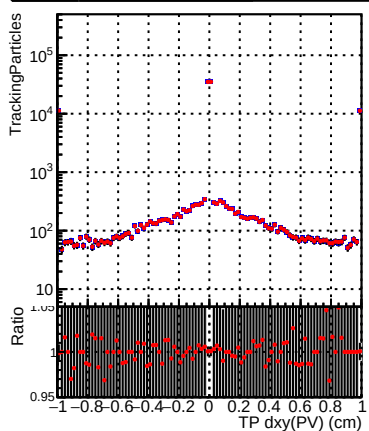
N of sim DQM_CKF_TTbase DQM_CKF_TT_retrainOldFiles125_v2_prelimWP_epoch4
