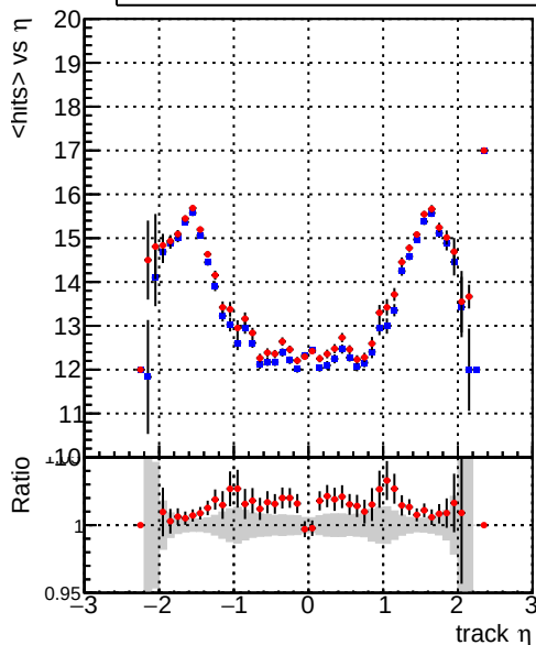
mean hits vs \eta — DQM_CKF_TTbase — DQM_CKF_TT_retrainOldFiles125_v2_prelimWP_epoch4
