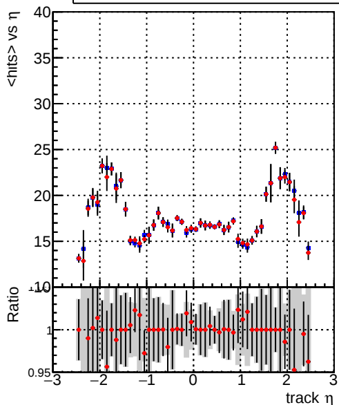
mean hits vs \eta Legend: DQM_CKF_TTbase (blue line), DQM_CKF_TT_retrainOldFiles125_v2_prelimWP_epoch4 (red line)
