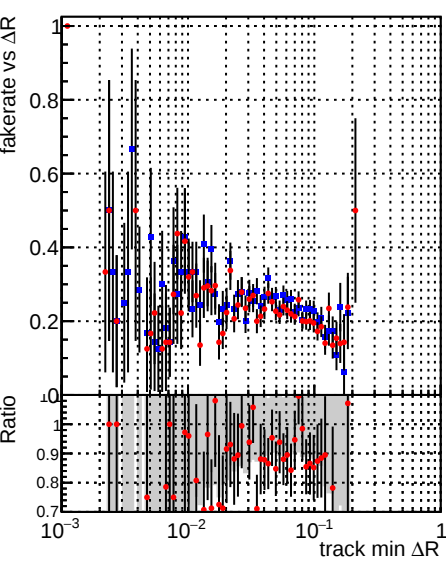
Legend: DQM_CKF_TTbase (blue), DQM_CKF_TT_retrainOldFiles125_v2_prelimWP_epoch4 (red)
