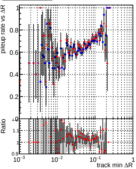
Legend: DQM_CKF_TTbase (blue), DQM_CKF_TT_retrainOldFiles125_v2_prelimWP_epoch4 (red)
