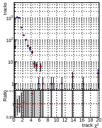
N of reco track vs. \chi^2 —●— DQM_CKF_TTbase —●— DQM_CKF_TT_retrainOldFiles125_v2_prelimWP_epoch4
