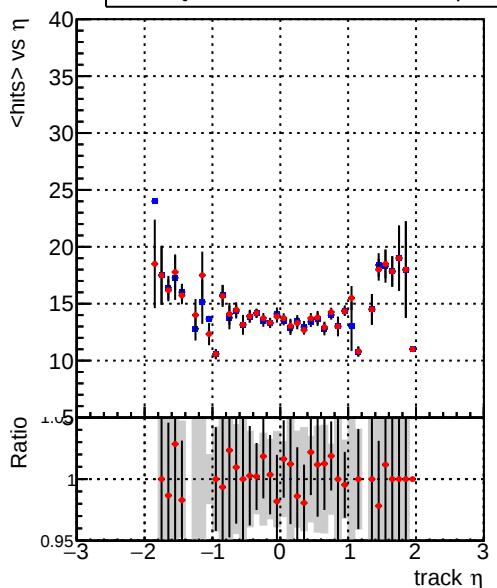
mean hit — DQM_CKF_TTbase — DQM_CKF_TT_retrainOldFiles125_v2_prelimWP_epoch4
