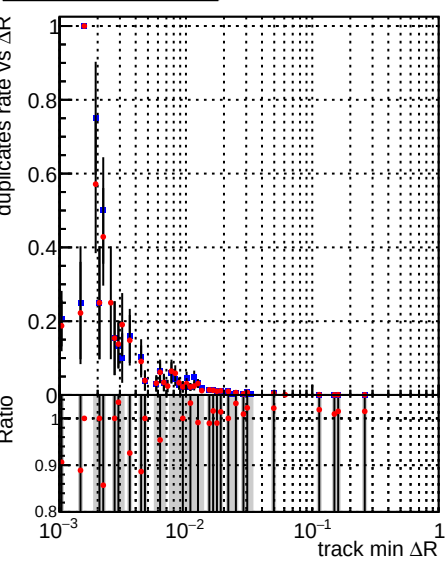
Legend: DQM_CKF_TTbase (blue squares), DQM_CKF_TT_retrainOldFiles125_v2_prelimWP_epoch4 (red circles)
